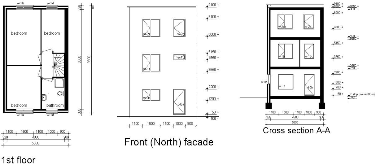
Figure 1: Some views of the test dwelling.
