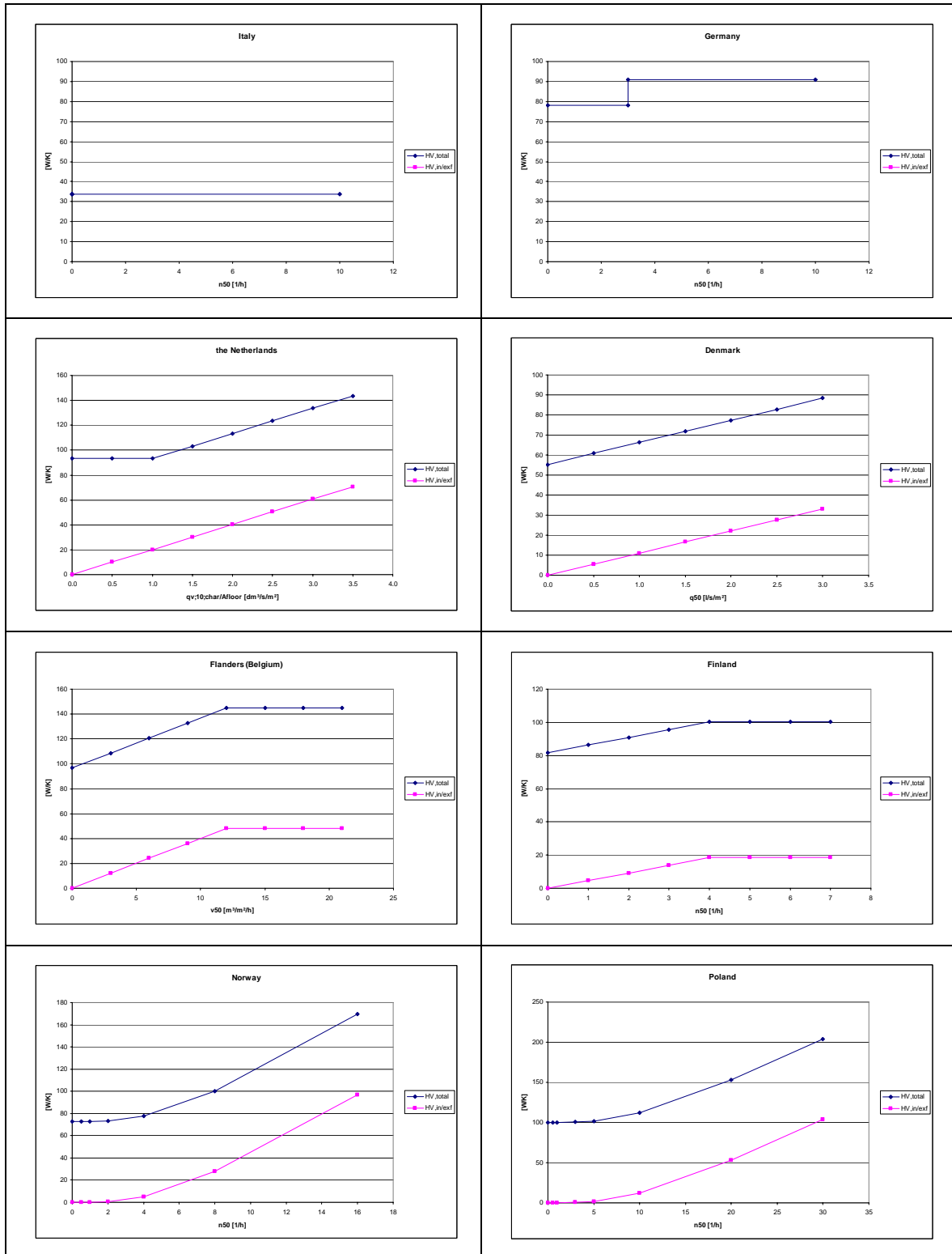
Figure 2: The total ventilation heat transfer coefficient and (if possible) the part of in/exfiltration in it as a function of the national airtightness indicator for 8 countries.
